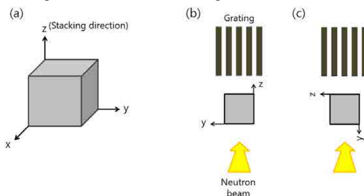
Fig. 1. (a) Coordinate system of the sample. (b) Measurement configuration for scattering in the y-direction. (c) Measurement configuration for scattering in the z-direction.
