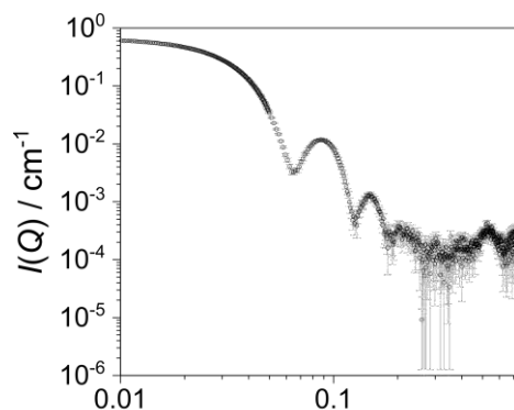
Figure 2. Small-angle X-ray scattering profile of the iron storage protein
