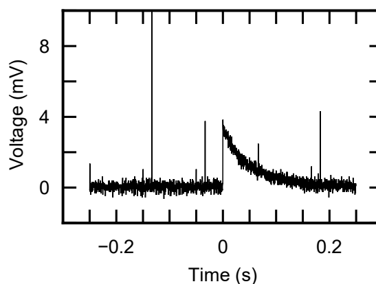
Fig. 1. Waveform of the X-ray induced signal obtained with an InGaP solar cell.
