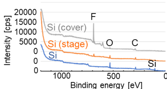
Fig. 2. XPS spectra for Si and CHF 3 -plasma-treated Si positioned on the sample stage or the cover of the plasma chamber.
