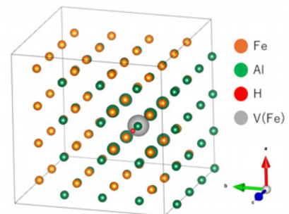
Fig. 1. Calculated atomic position of hydrogen trapped by Fe vacancy in Fe-Al alloy.
