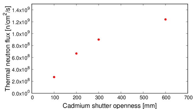
Fig. 1. Relationship of the thermal neutron flux and the cadmium shutter openness.
