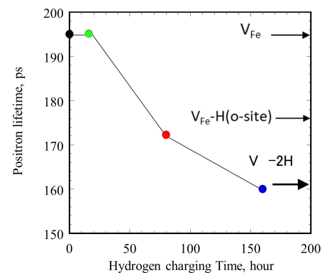
Fig. 2. Positron annihilation lifetime in hydrogen charged Fe-Al measured with 4 keV positrons and calculated values of H-V complexes.
