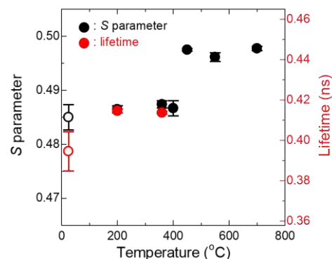
Fig. 2. Dependence of S-parameter and Positron annihilation lifetime on rising temperature.
