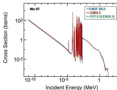
Fig. 1. Cross-section of Mo-97
