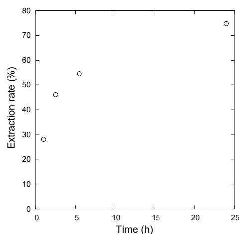
Fig. 2. Extraction rate of ^{99}\text{Mo} to water
