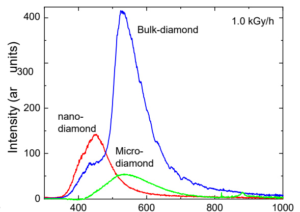
Fig. 1. Gamma-ray-induced luminescence spectra of nano, micro, and bulk diamonds measured at room temperature with an absorbed dose of 1.0 kGy/h.
