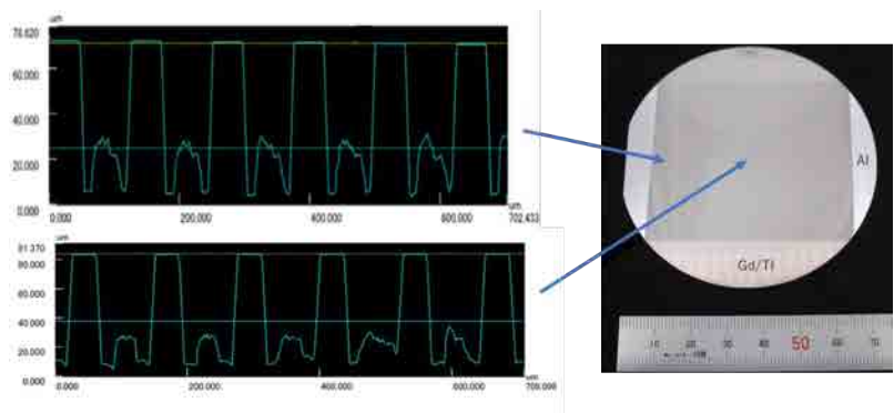
Fig.1 Groove depth of different parts of the micro-cut G0 grating.
