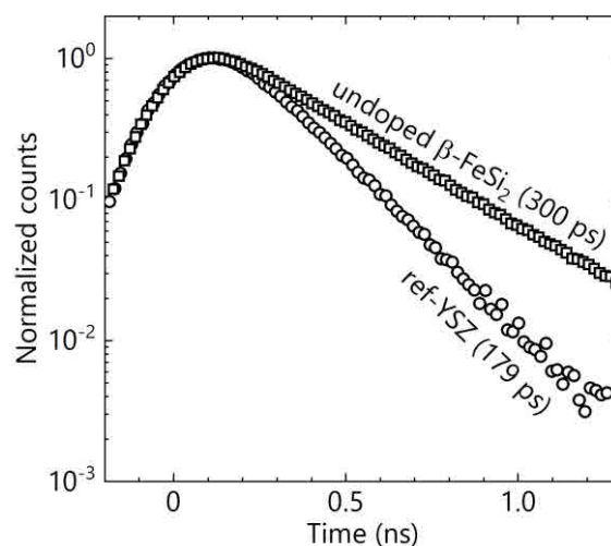
Fig2. Measured positron annihilation lifetime spectra of reference YSZ and the \beta -FeSi film.
