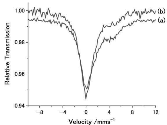
Fig. 1. ^{197}\text{Au} Mössbauer spectra at 20 K for the sample of Au(III) adsorbed on MnO 2 . (a) prepared from acid solution, (b) from alkaline.
