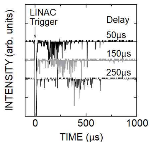
Fig. 1 Positron signals recorded for different delay times of the linear storage.
