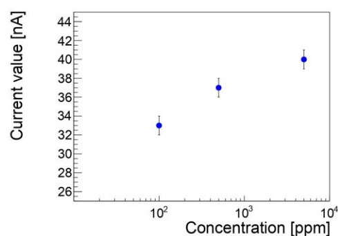
Fig. 1. Current value from scintillation signal as a function of concentration of ^{10}\text{B} in the target sample.
