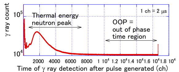
Fig. 1 Time spectrum of \gamma ray detection.
