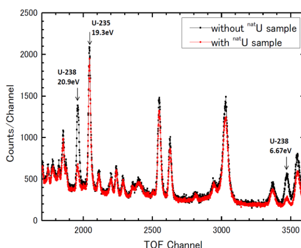
Fig. 1 Comparison of the TOF spectra for prompt gamma-rays from the HU indicator with and without natural uranium sample
