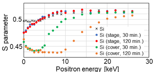
Fig. 1. S-parameters of Si and CHF 3 -plasma-treated Si positioned on the sample stage or the cover of the plasma chamber, exposed for 30 or 120 min.
