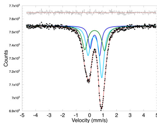
Fig. 1. Mössbauer spectra of hornblende single crystal under γ-ray //a-axis and a peak separation with three OS doublets.
