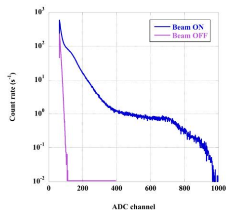
Fig. 2. Results of neutron survey meter measurements.
