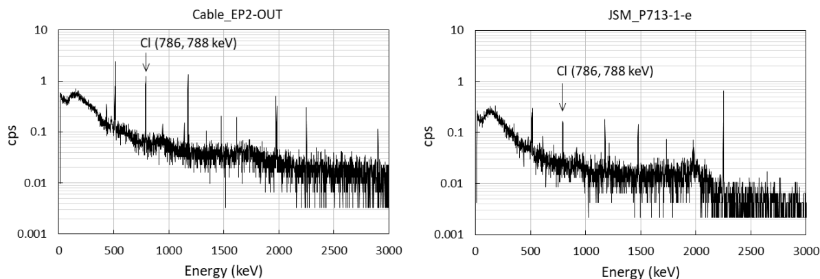
Fig. 1. Prompt \gamma -ray spectra of representative cable sheath sample (right) and standard (left)
