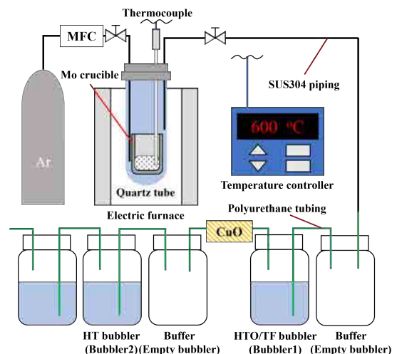
Fig. 1. Experimental apparatus.
