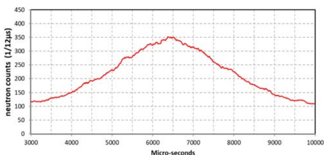
Fig. 2 A sample of the neutron count distribution at a rotation speed of 4000 rpm, in the presence of nuclear materials.
