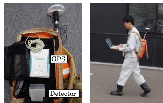
Fig. 2. KURAMA-II in a backpack.
