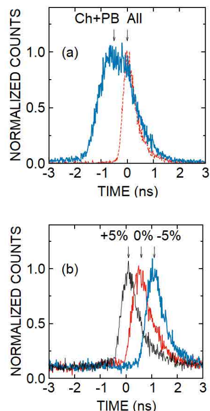
Fig. 1. Lifetime spectra to observe pulse shapes.
