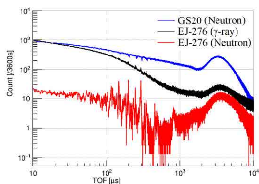
Fig. 2 Obtained TOF spectra of 3-mm-thick EU.
