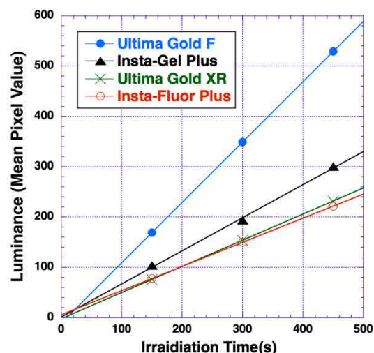
Fig. 1. Luminescence value for different types of boron-added liquid scintillators as a function of neutron irradiation time.
