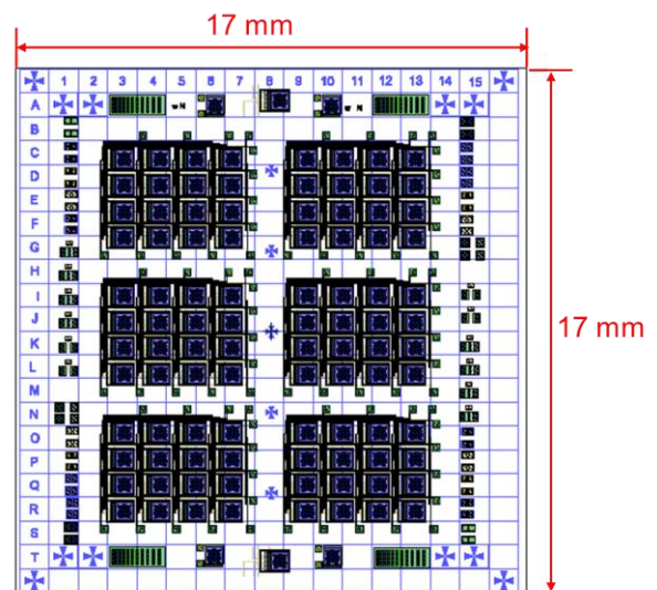
Fig. 1. Chip layout of the neutron CMOS
