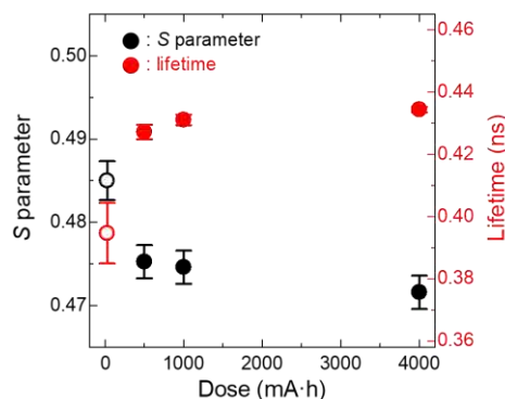
Fig. 1. Dependence of S-parameter and Positron annihilation lifetime on soft X-ray dose.
