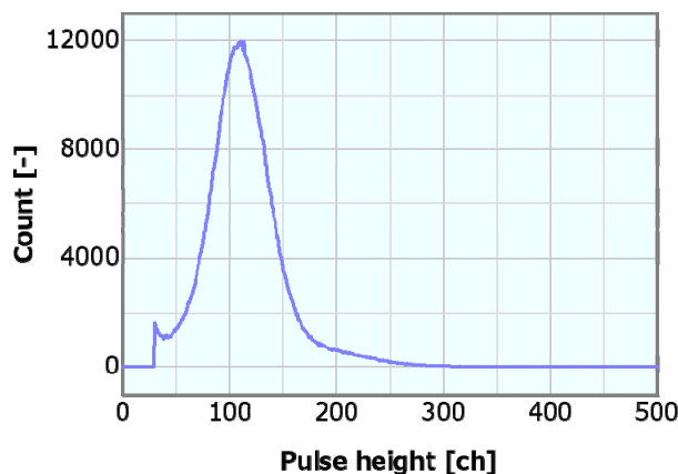
Fig. 1. Pulse height distribution of lithium glass scintillator.
