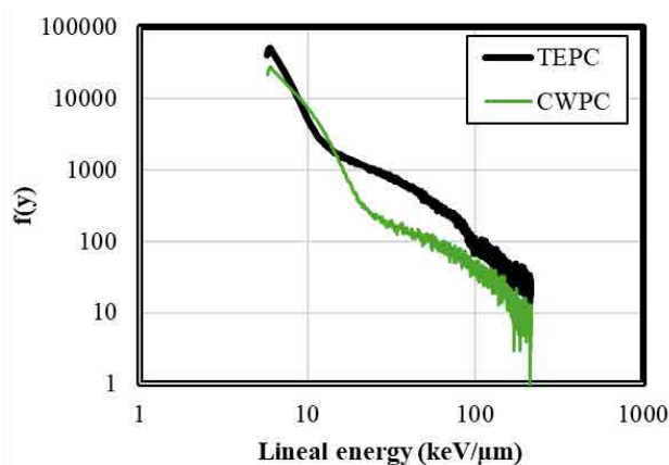
Fig. 1. Left) The frequency distribution curve of the KUR epithermal mode measured with the TEPC (black line) and CWPC (green line). Right) Image of the experimental set up.
