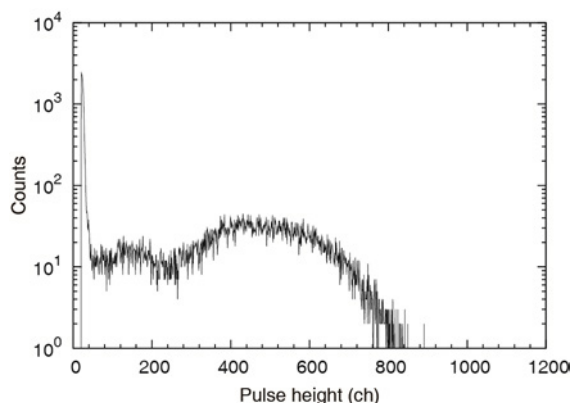
Fig. 1. Pulse height distribution of small LiCAF scintillator.
