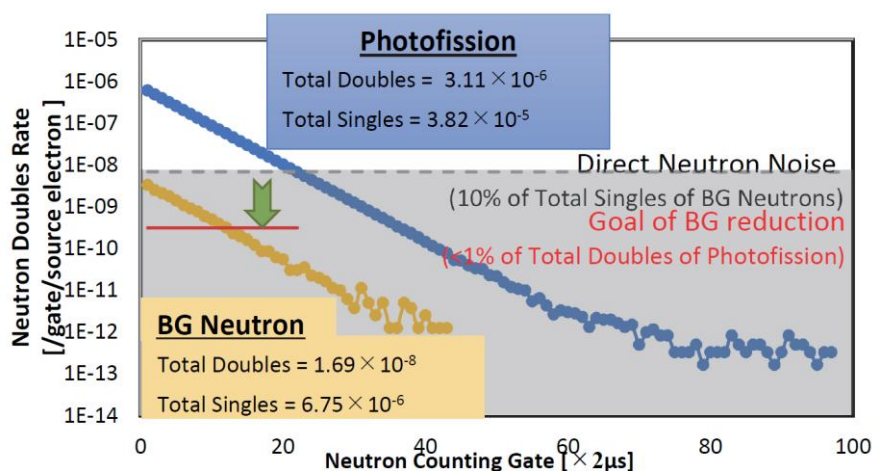
Fig. 1 Accidental neutron injection noise reduction goal.[1]
