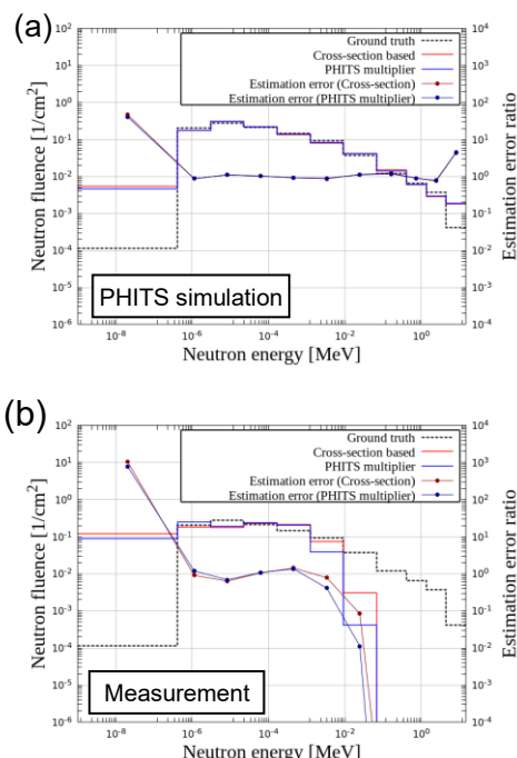
Fig. 2. Estimated neutron energy spectrum by SOF detector.
