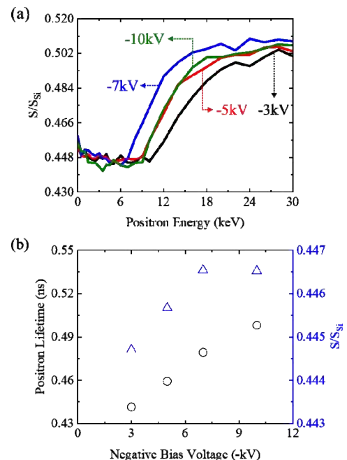
Fig. 1 (a) S-parameter depth profiles of F-DLC films. (b) bias voltage dependence of normalized S-parameter and positron lifetime at different bias voltages.
