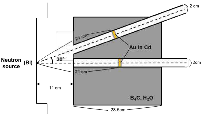
Fig.1 Device for measurement of C/F ratio.
