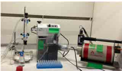
Fig.1. Extraction-chromatography set-up with on-line γ-ray detector for Yb/Lu separation.
