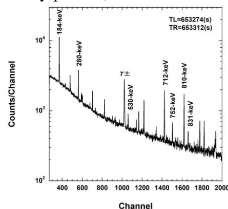
Fig.2 \gamma -ray spectrum of ^{166\text{m}}\text{Ho} .
