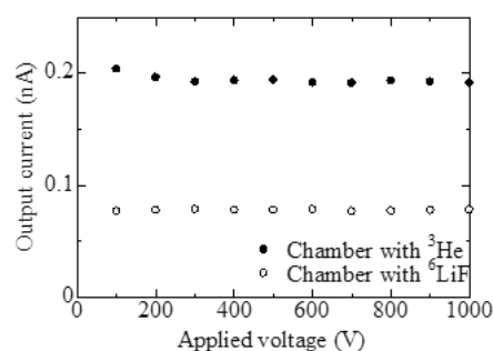
Fig. 2. Relation between applied voltage and output current.
