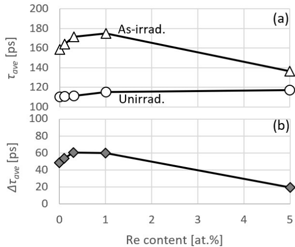
Fig. 1. Re content dependency of (a) average positron lifetime, (b) increase of average positron lifetime.
