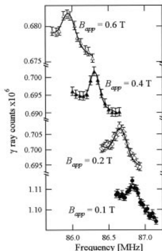
Fig. 1. NMR/ON resonances of ^{140}\text{LaFe} measured by detecting the 1596 keV \gamma -transition at B_{app} = 0.1, 0.2, 0.4 , and 0.6 T.
